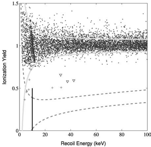
Figure 10 Ionization yield y versus recoil energy for WIMP-search data for three Ge detectors (total mass 0.75 kg) with a raw live time of 53 days from the CDMS II experiment (net exposure, after cuts, in 19.4 kg-days) (84). WIMP-search events for ionization yield, y > 0.75 , are shown as points, y < 0.75 as geometrical shapes. The expected region for WIMP nuclear recoil events lies between the two lower dashed lines. The y value for the nuclear recoil events has a slight slope due to the energy dependence of the nuclear recoil quenching factor in Ge.
